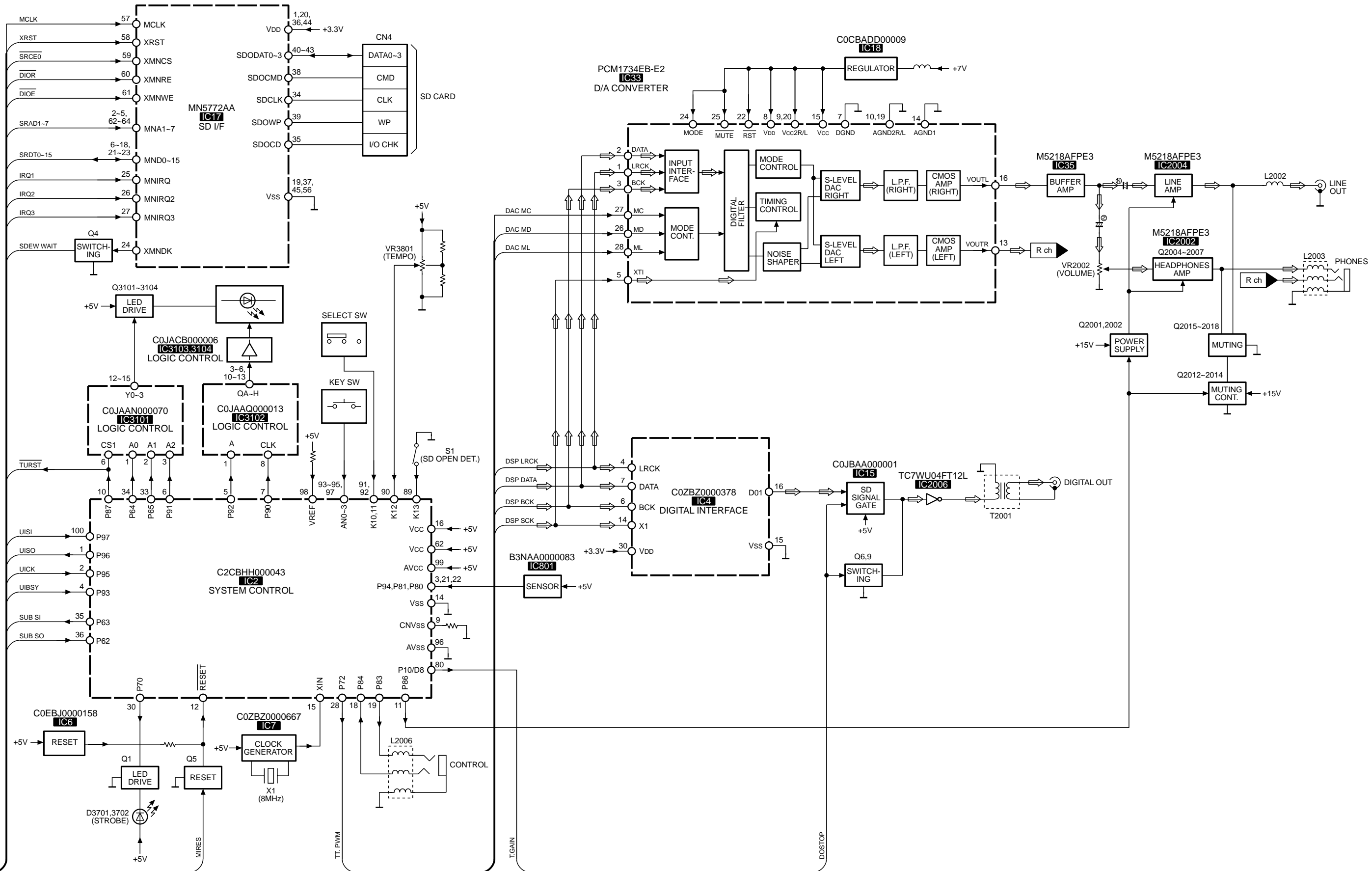
SL-DZ1200(PP,EB,EG,EP,GN) BLOCK DIAGRAM
